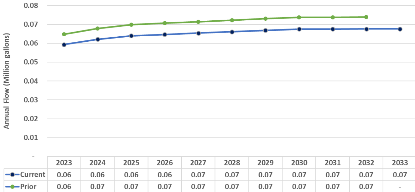
Seis Lagos Wastewater Treatment Plant Flow Comparison
